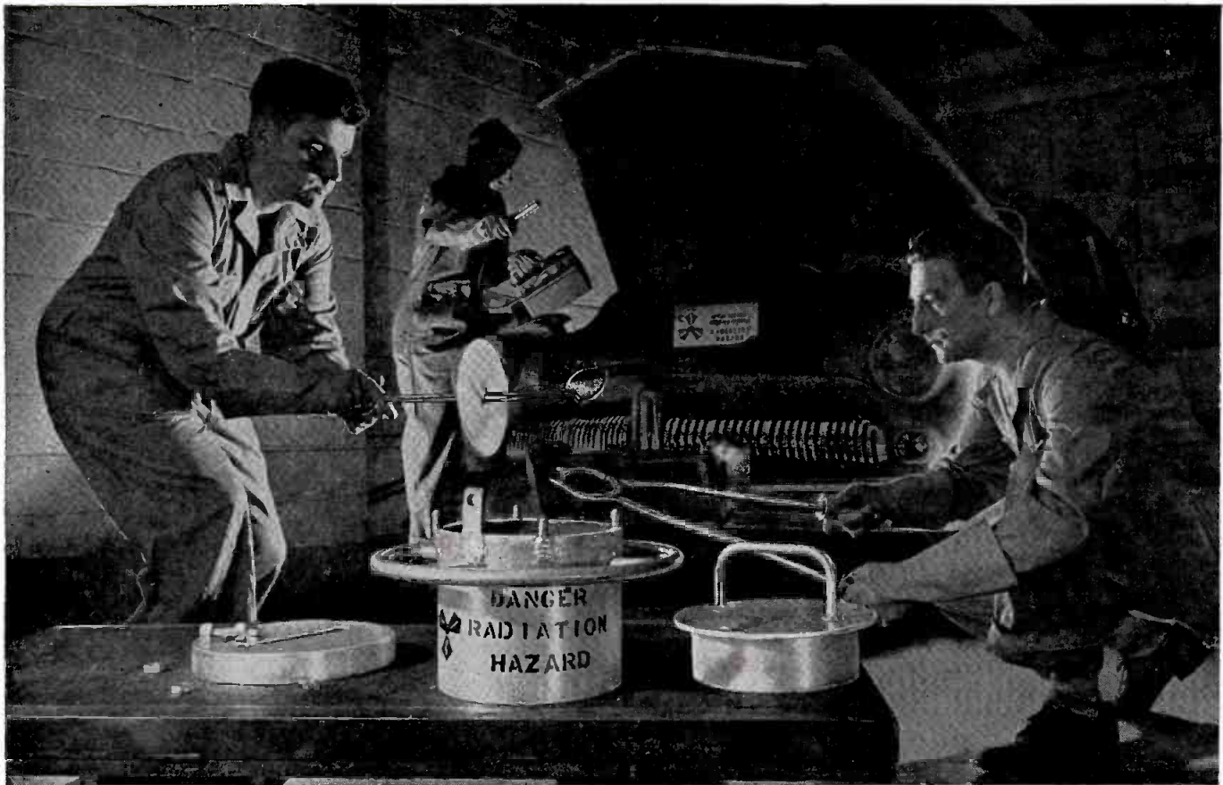
PISTON RING MADE RADIOACTIVE in Atomic Pile at Oak Ridge, is carefully installed in test car engine by specially trained scientists. Radioactivity is checked with Geiger counter at all times. Car is then driven in proving
